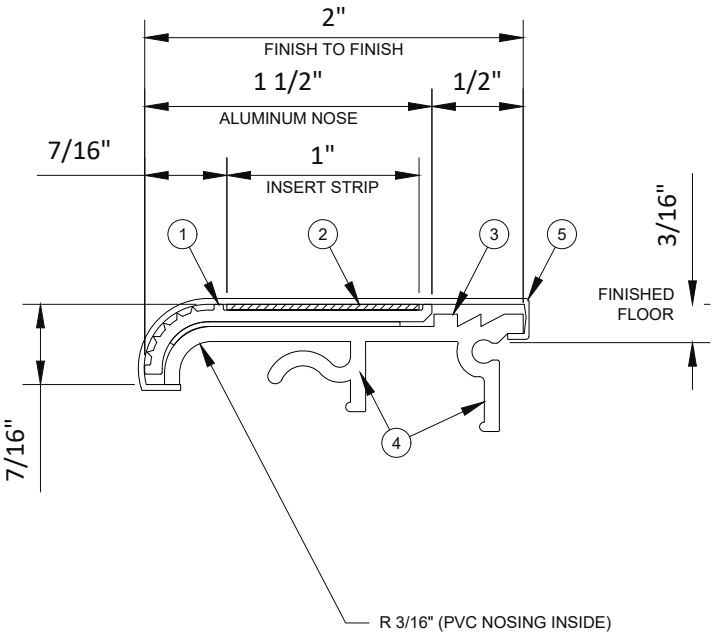
A NOSING ASSEMBLY DETAIL
