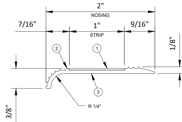
A NOSING ASSEMBLY DETAIL
