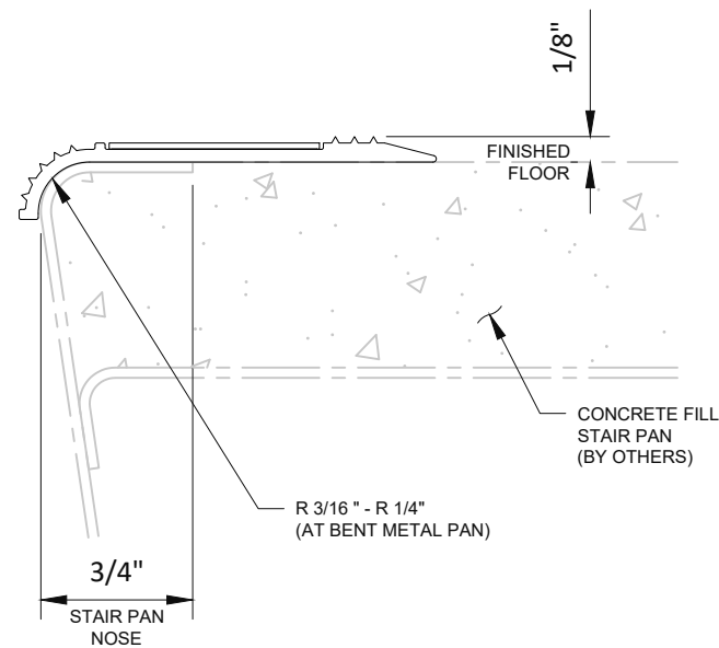
D2 SURFACE MOUNT CONCRETE PAN FILLED STAIR INSTALL (LIQUID ADHESIVE ATTACHMENT)
