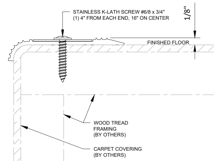
D4 SURFACE MOUNT CARPET STAIR INSTALL (SCREW ATTACHMENT)
